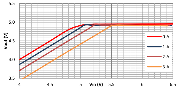
Figure 12. SCT2331 LDO Mode Waveform
