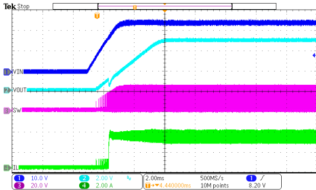
Figure 16. Power Up VIN=24V, VOUT=5V, IOUT=3A
